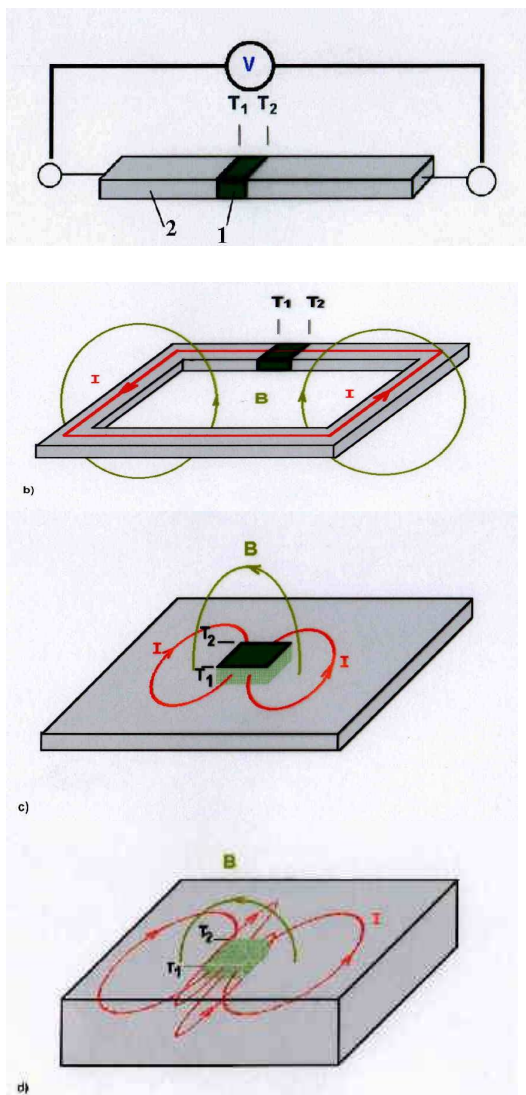
Figure 1: Different geometries containing metal 1 and metal 2 with temperatures T_1 and T_2 at their interfaces. According to the Seebeck effect a voltage V , currents I and magnetic fields, here depicted as magnetic flux density B , are generated.
