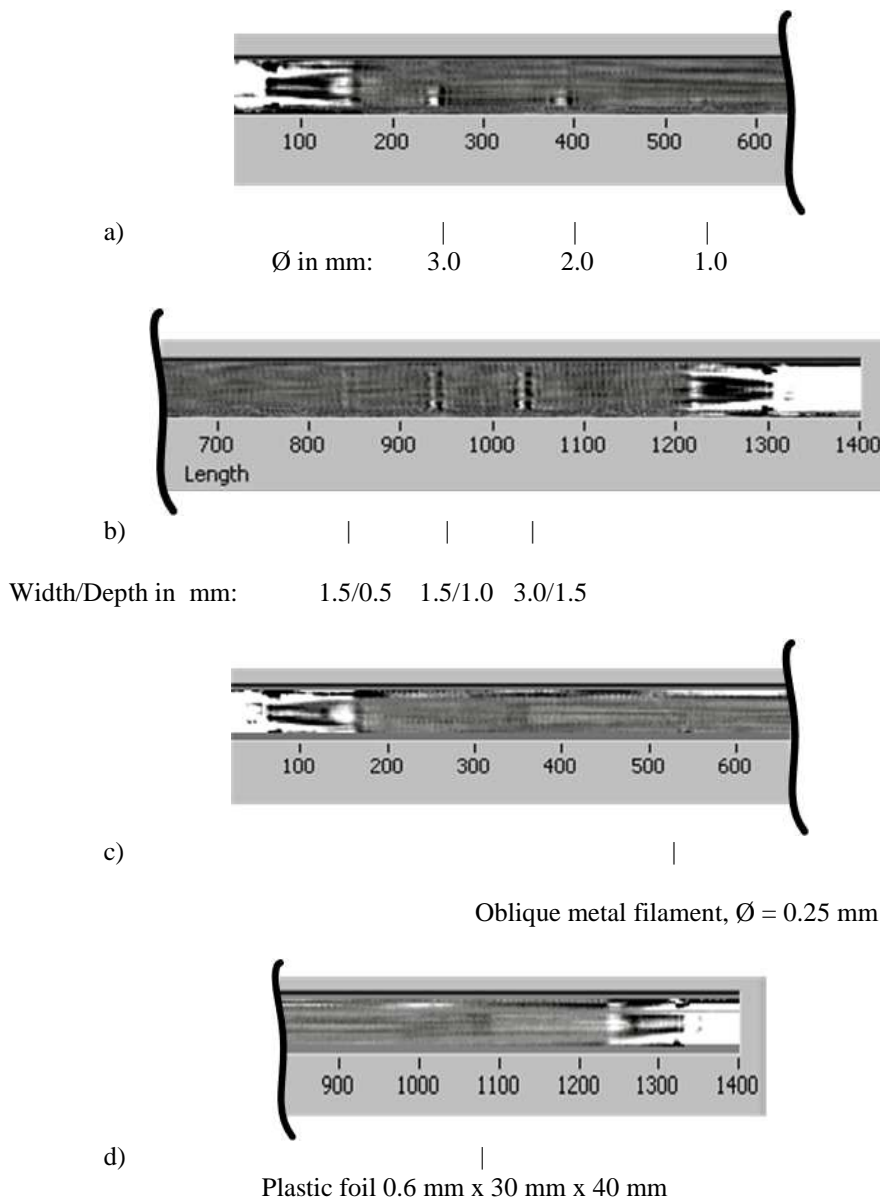
Figure 2: Microwave Scans of Leaf Springs with Artificial Defects. a) Transversal Bore Holes b) Grooves. c) Metal Filament. d) Plastic Foil
